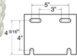
Mounting Plate
