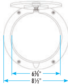
Over-sized PVB-85CVR
