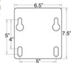
Mounting Plate
